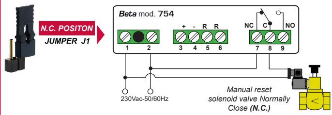
Fig. 5 Application example with Manual Reset solenoid valve Normally Close.
