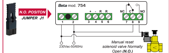
Fig. 4 Application example with Manual Reset solenoid valve Normally Open.
